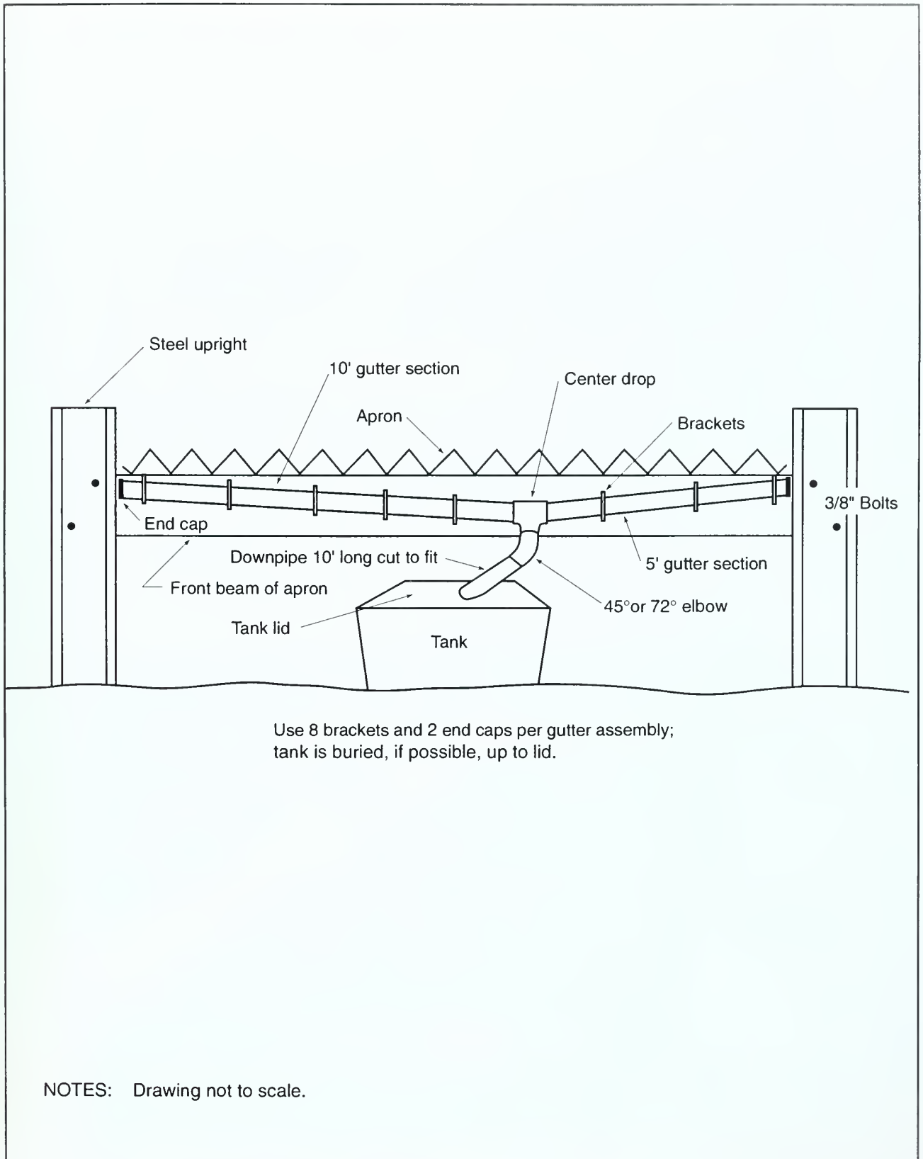
Figure 6. Carson City BLM big game guzzler gutter details.
